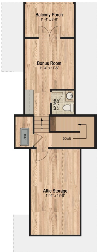
Floor Plan - 2nd Floor
